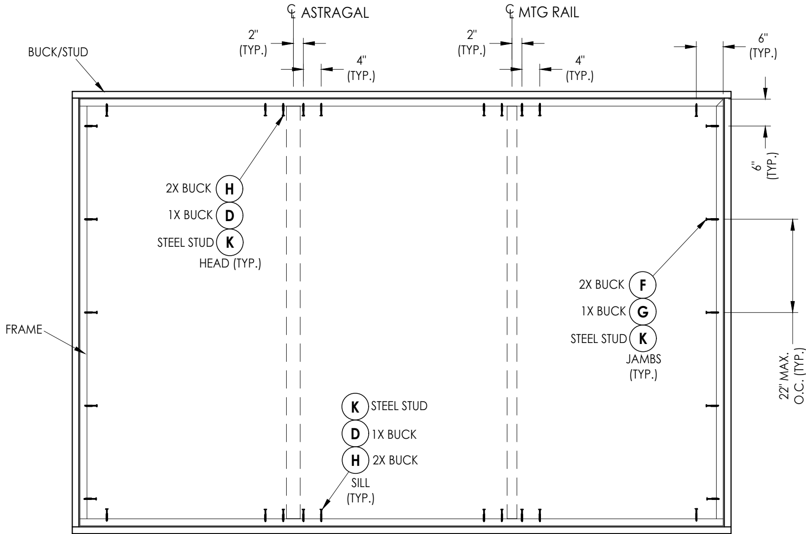
FRAME ANCHORING
