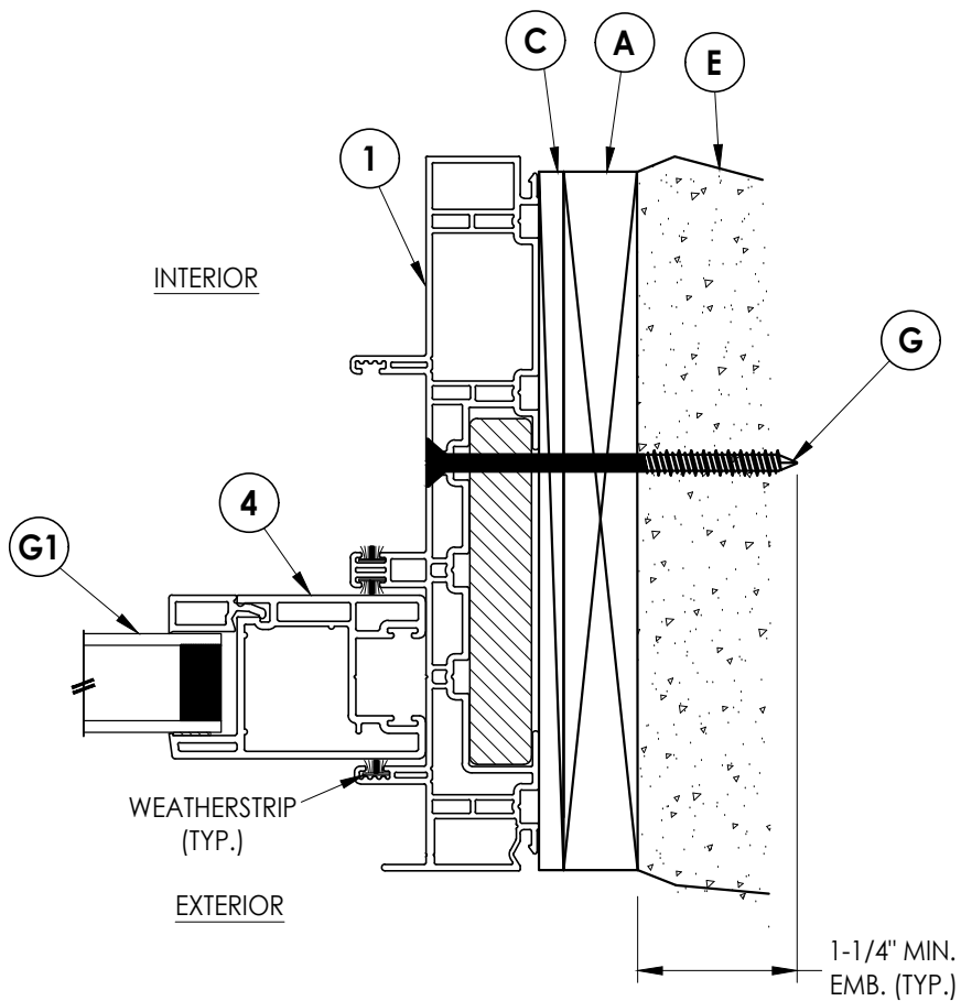
3 2 HORIZONTAL CROSS SECTION Shown w/ 1X Buck Construction
