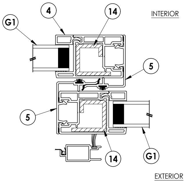
2 2 HORIZONTAL CROSS SECTION Shown w/ 2X Buck
